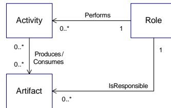
Fig.5. Process description metamodel
