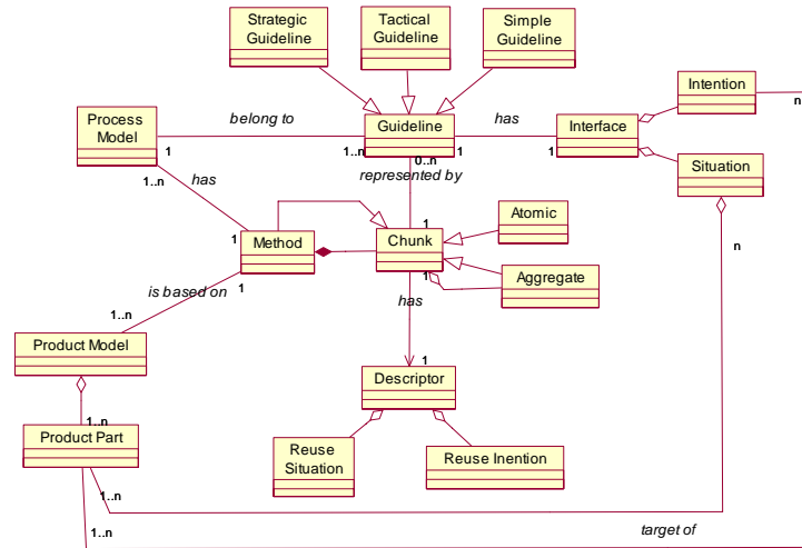
Fig. 1. The metamodel of the chunk (redrawn from [22])
