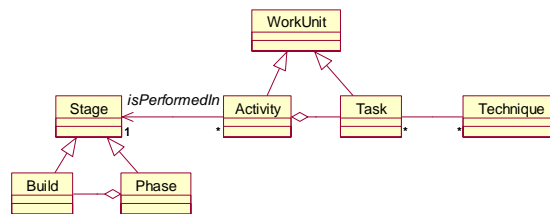
Fig. 3. WorkUnit (process) elements (redrawn from [11])
