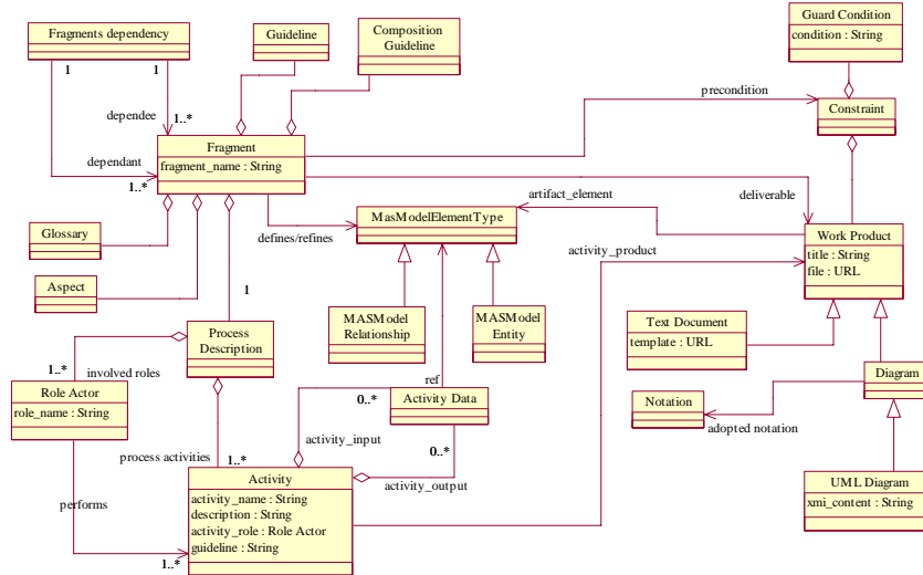
Fig. 6. The metamodel of the FIPA method fragment
