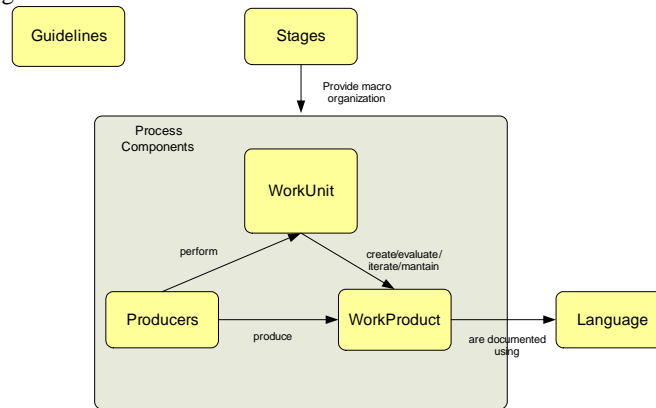
Fig. 2. OPF MetaModel (redrawn from [6])
