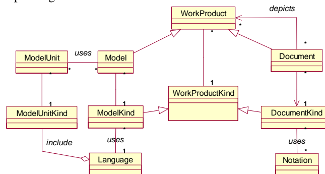
Fig. 4. Work Product elements (redrawn from [11]).
