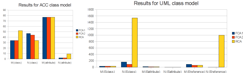
Fig. 8. Results for ACC class model
