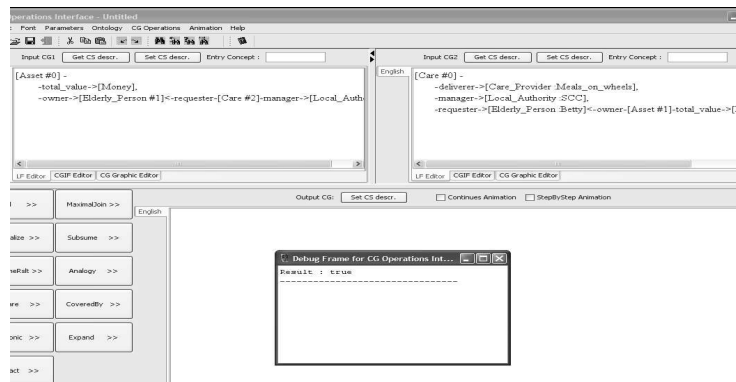
Fig. 12. Successful Projection of Rule into Fact.
