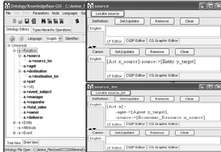
Fig. 7. Developing a TM Conceptual Catalogue in Amine.
