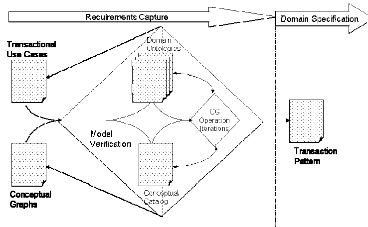
Fig. 2. TrAM, with automation.
