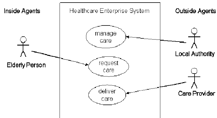
Fig. 3. Transactional Use-Case.
