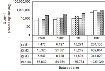
(a) Query1 (BSBM)
