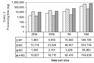
(c) Query2 (BSBM)
