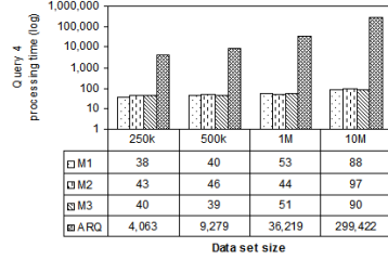
(b) Query4 (SP 2 B)
